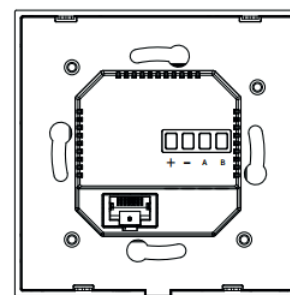
4 BACK VIEW
