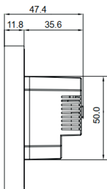
2 RIGHT VIEW
